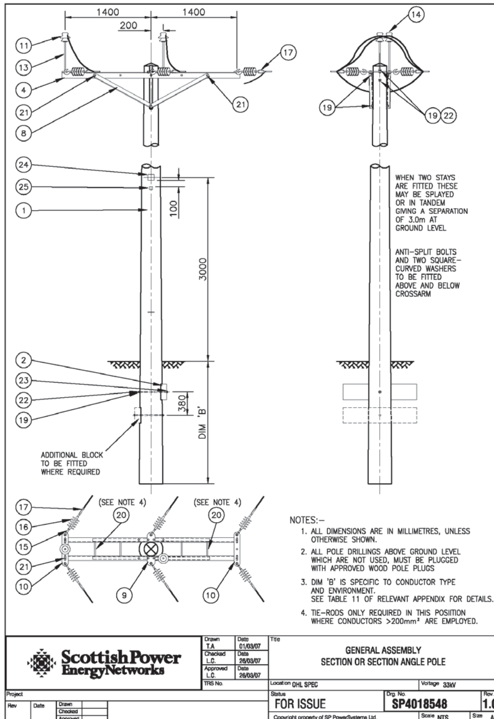
Figure 12 Single Pole Straight Line or Angle Section (Drawing SP4018548)
